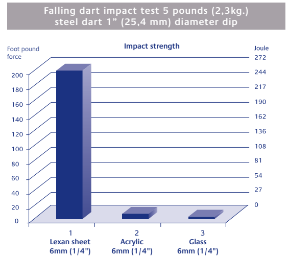
Figure 1 Impact resistance
