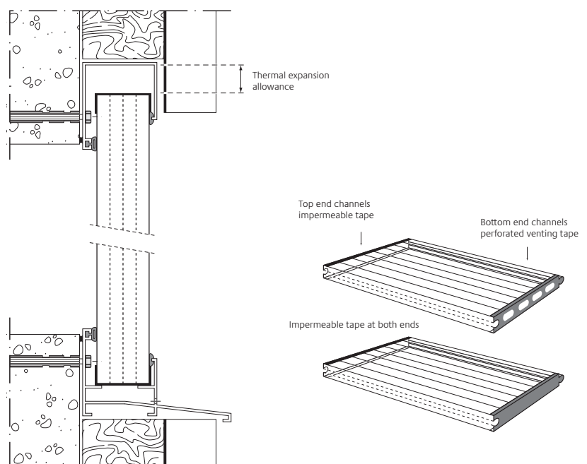
*Typical glazing detail Thermoplastic/alu glazing profile
